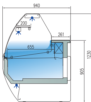
CV-9-10-C CV-9-13-C CV-9-15-C CV-9-20-C CV-9-25-C CV-9-30-C
