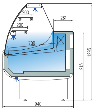
CVEP-9-10-C CVEP-9-13-C CVEP-9-15-C CVEP-9-20-C CVEP-9-25-C CVEP-9-30-C
