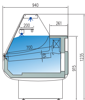
CVE-9-10-R-P CVE-9-13-R-P CVE-9-15-R-P CVE-9-20-R-P CVE-9-25-R-P CVE-9-30-R-P
